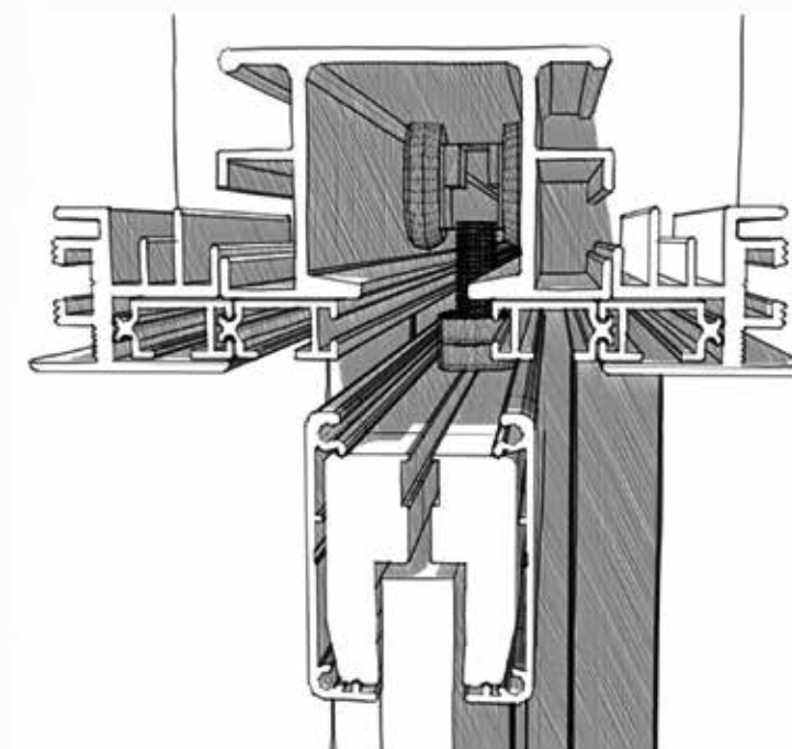
Sliding door "MODULAR RASO" Frame without cover-joint adaptable to standard counterframes Single door Mod. Transparent_TRANSPARENT Collection
