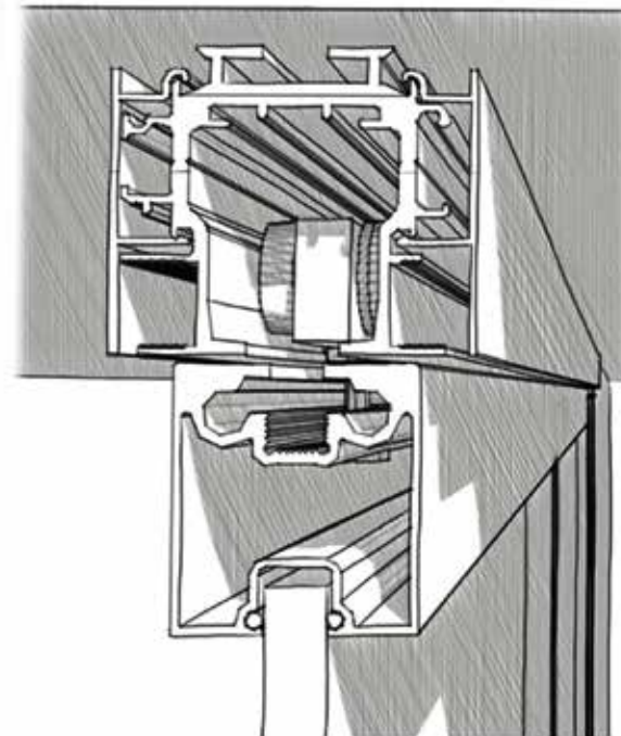
Asymmetrical folding sistem Five doors panel "LUMAN" three folding right and two left
